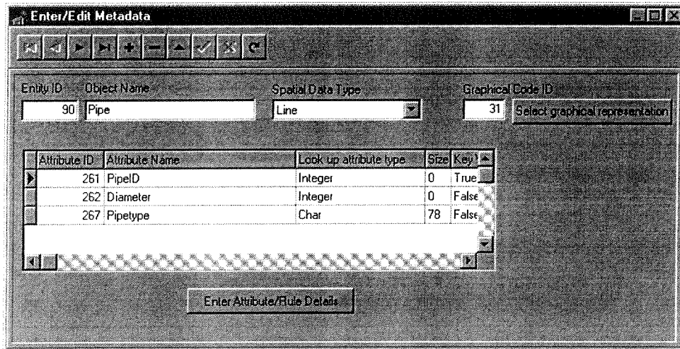
Figure 6 Metadata Entry
