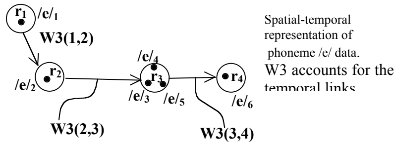
Fig.5a Consecutive phoneme data frames cause creation of links between the rule nodes.
