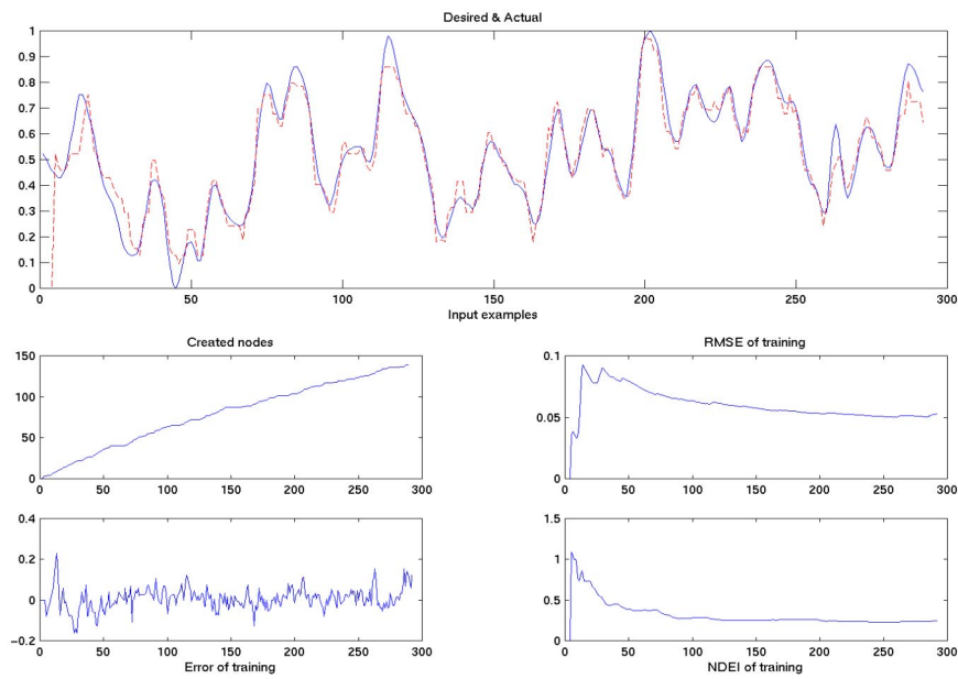
Fig. 14c EFuNN is trained on the first half of the data and tested on the whole data set (either in an on-line or in an off-line mode)
