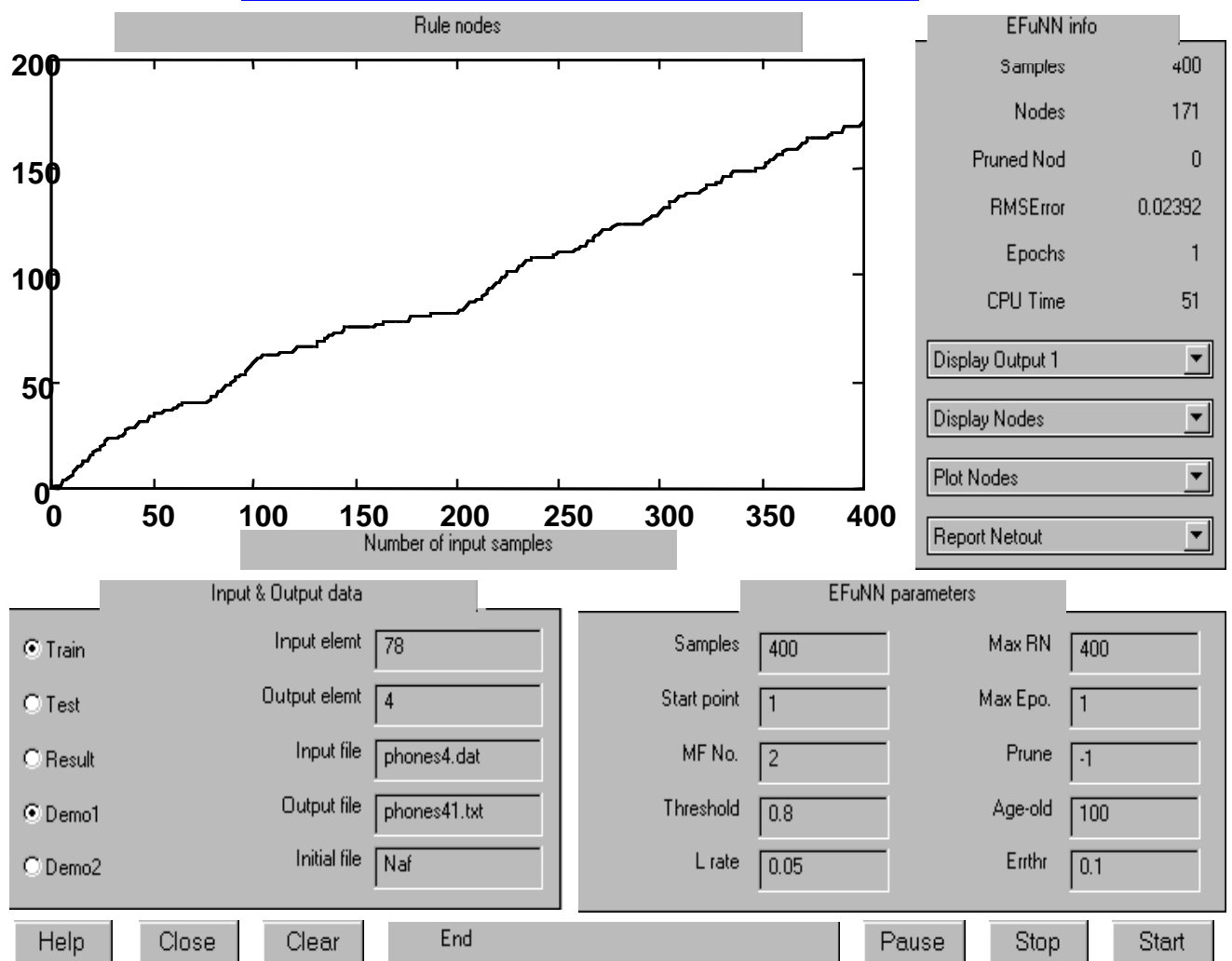
Fig. 7a shows the growth of the number of the rule nodes with the progress of entering data examples for one pass of training and the root mean square error RMSE.
