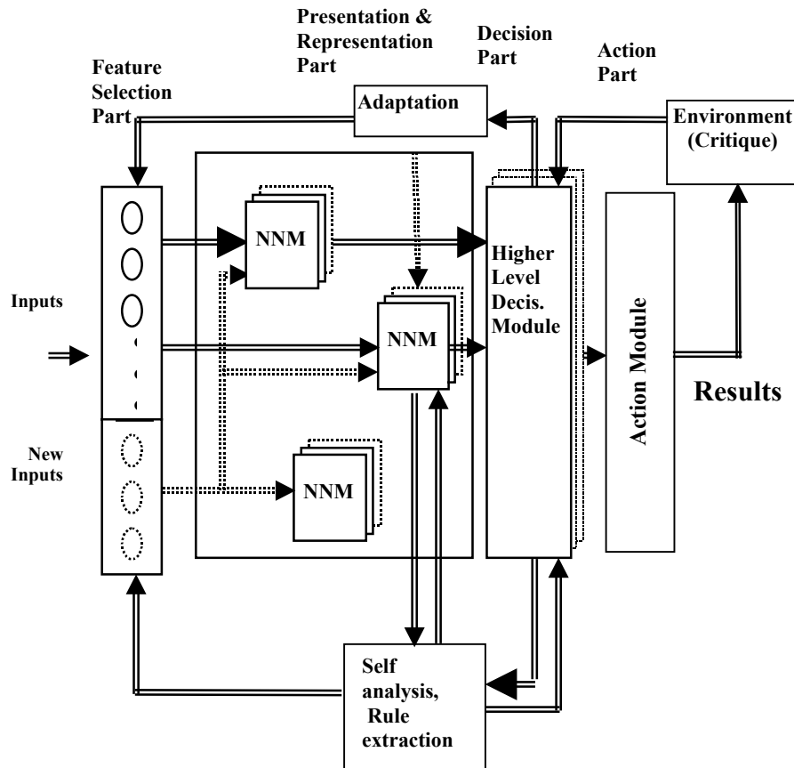
Fig.1 Block diagram of the ECOS framework.
