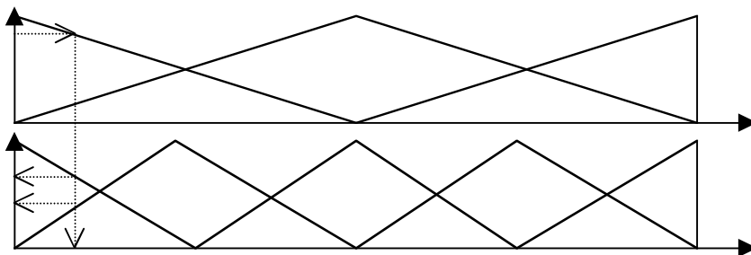
Fig. 10c The number of the MF increases from 3 to 5;
