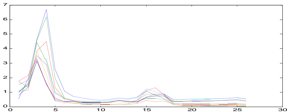
Fig. 11a Phoneme /I/ from ‘sit’- 10 consecutive mel scale vectors, each of 26 elements;
