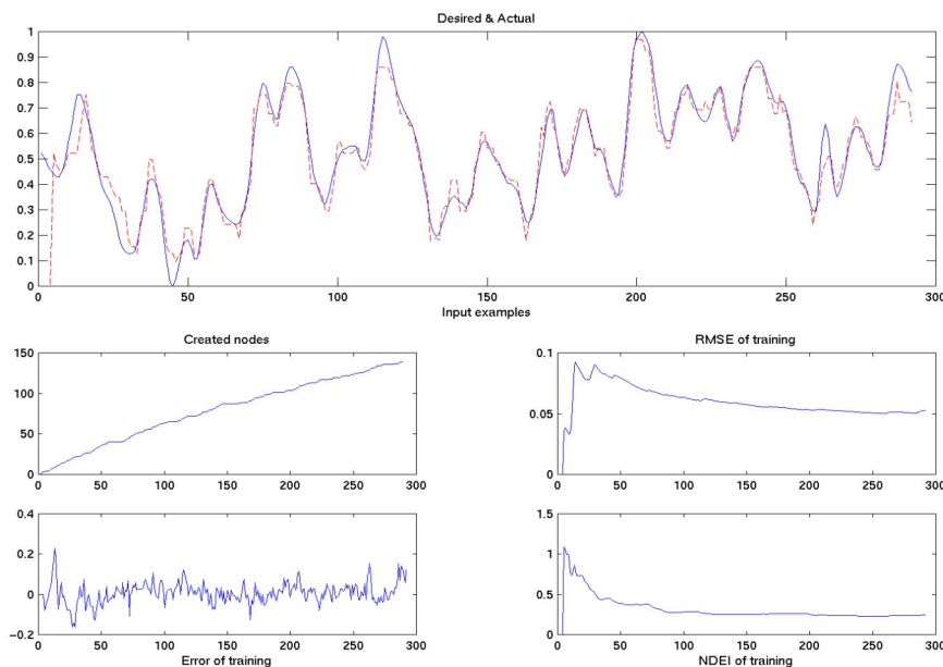
Fig.14a EFuNN is trained on each data item in an on-line mode and tested immediately to predict the following data item before it is accommodated in the system.
