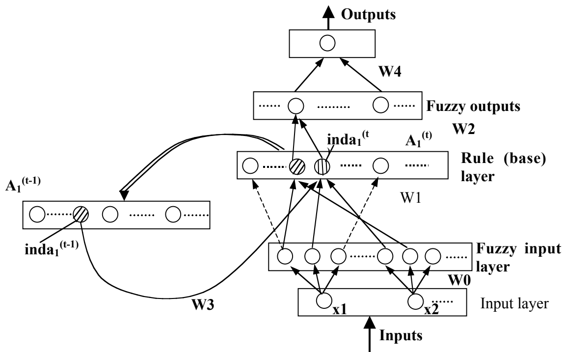
Fig2b EFuNN with a short term memory and a feedback connection
