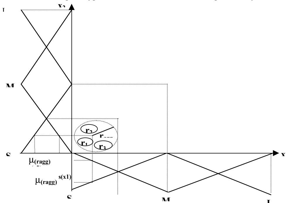
Fig8b The process of aggregation of three rule nodes r1, r2 and r3 into one cluster node r_{agg} ;
