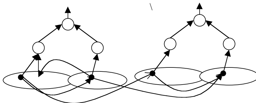
Fig.6. Different strategies for rule node insertion and connection creation
