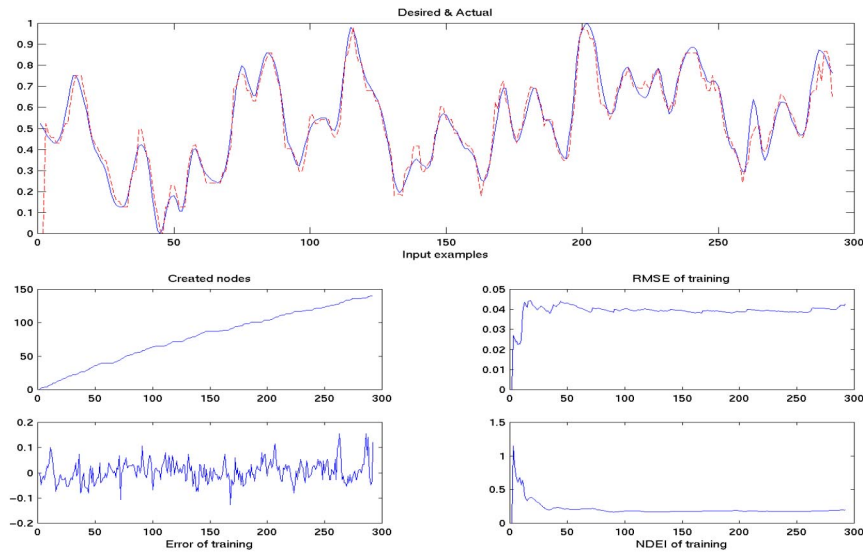
Fig.14b EFuNN is trained on each data item in an on-line mode and tested immediately to predict tree steps ahead data item
