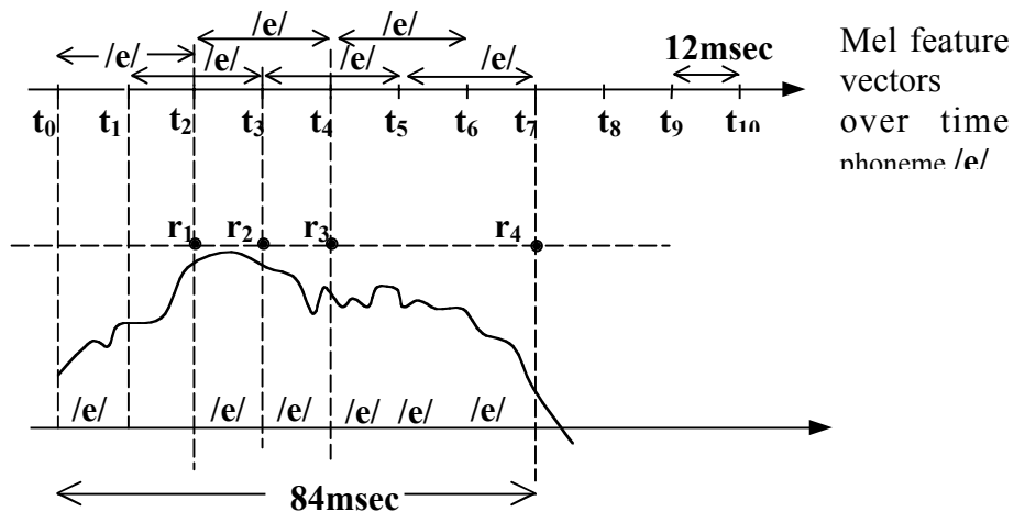
Fig.5b Schematic diagram of the raw phoneme data and the points in time of rule node creation.
