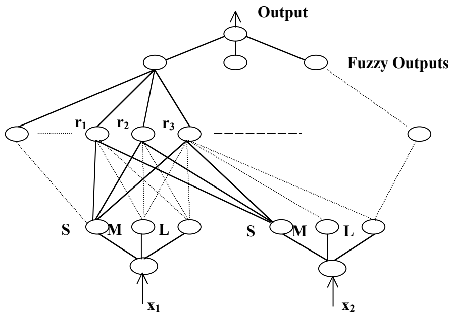
Fig.8a An evolved EFuNN structure;
