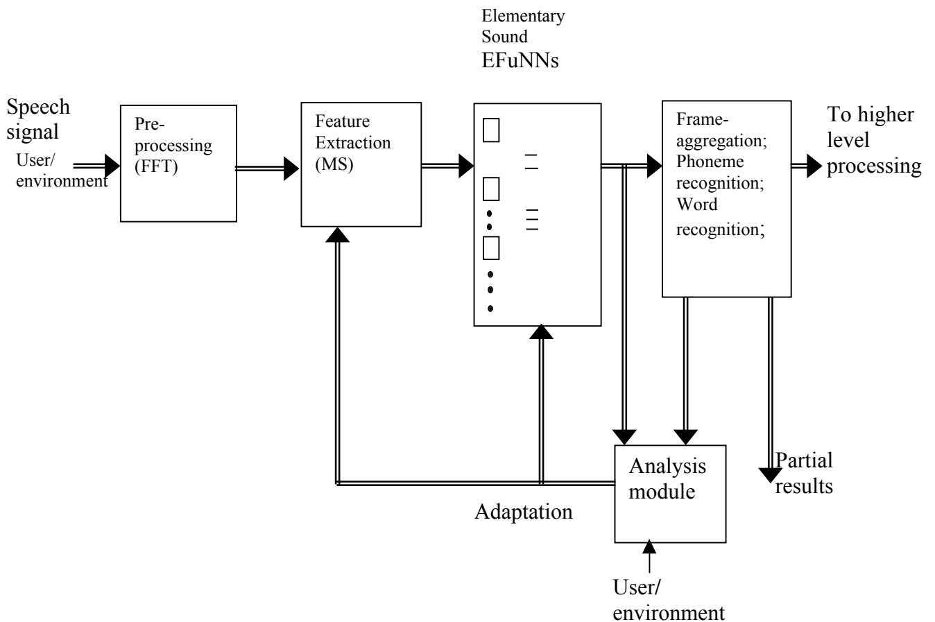
Fig.13. A block diagram of an ECOS and EFuNN-based adaptive speech recognition system where the phoneme modules adapt to new data in an on-line mode during the operation of the system
