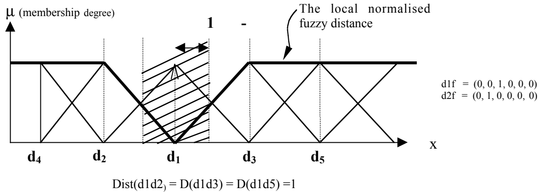
Fig.3. Membership functions (MF) and the local, normalised, fuzzy distance function
