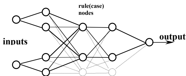
Fig.2a The five layers basic structure of the EfuNNs.
