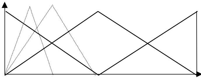
Fig. 10a New MF are inserted without modifying the existing ones.
