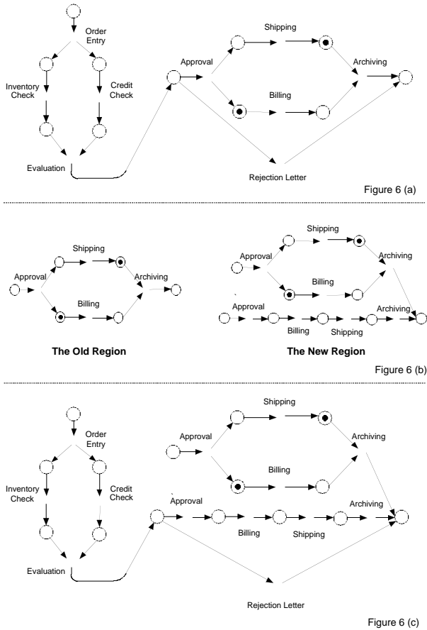
Figure 6. An adaptive Petri net example
