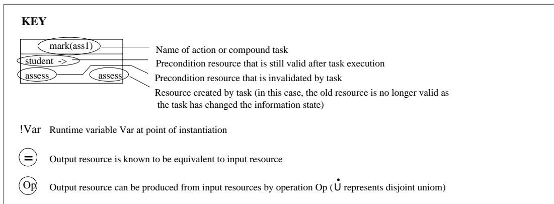
Figure 4: An example plan (the bold node is an unexpanded compound task)
