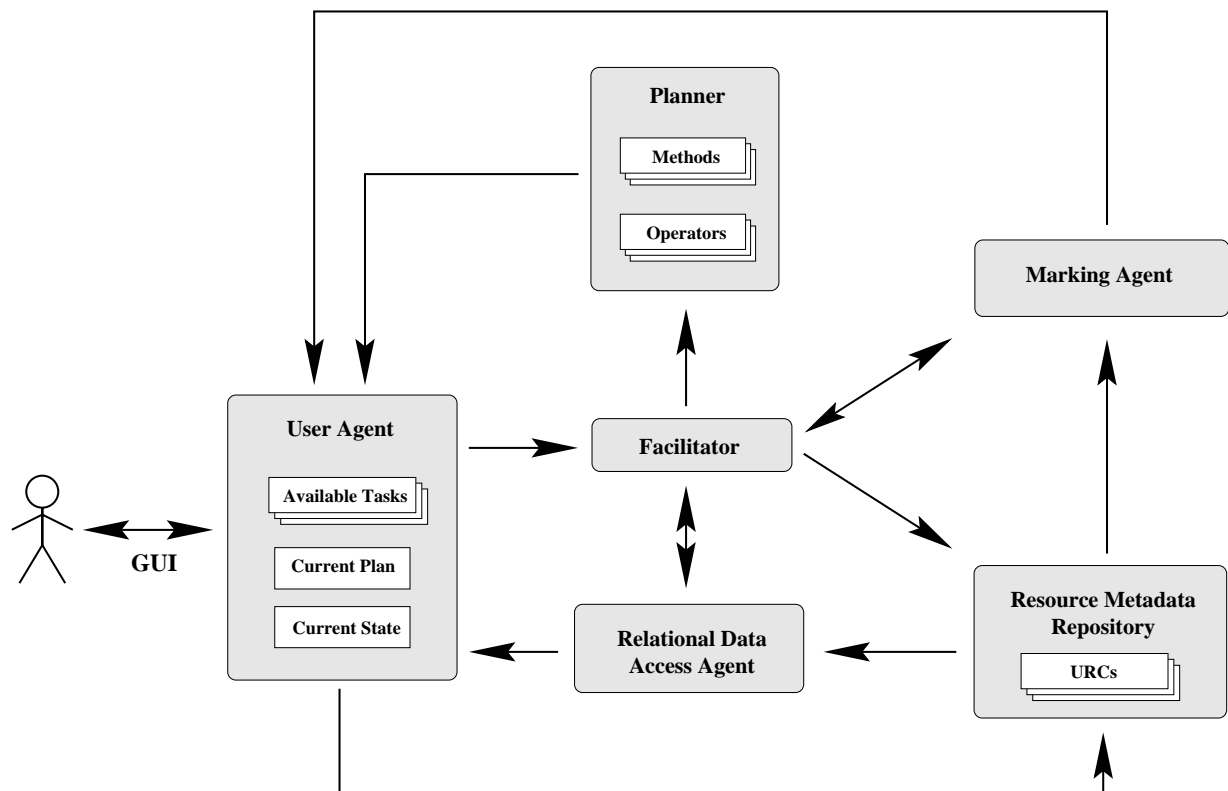
Figure 1: The prototype system architecture
