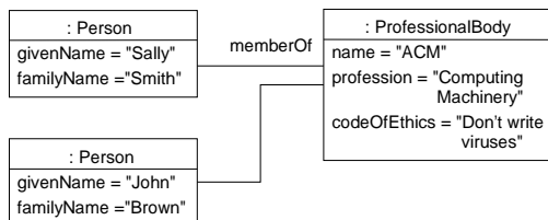
Figure 3: A simple UML object diagram example
