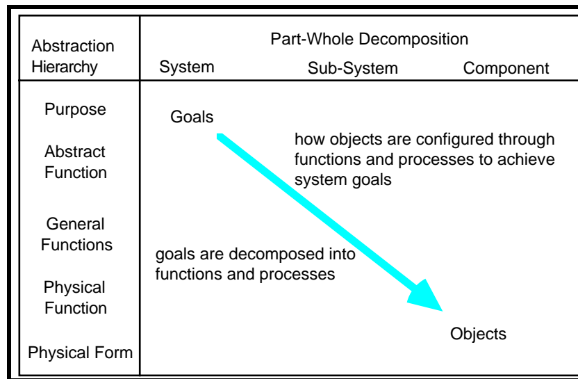
Figure 1 The Abstraction Hierarchy and the Part-Whole Decomposition shows the relationship between form and function in a work domain.
