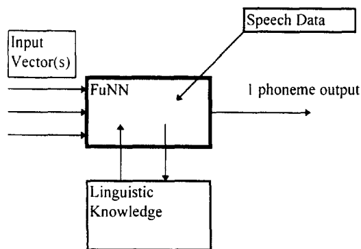
Fig. 11. The use of a FuNN module for a single phoneme recognition.
