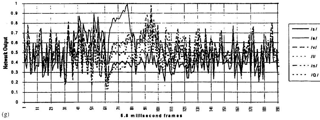
Layer One Neural Networks, Outputs for "seven" (Experiment 2)
