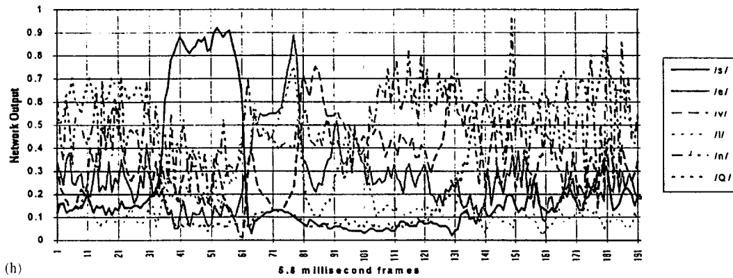
Layer Two Neural Network, Output for "seven"
