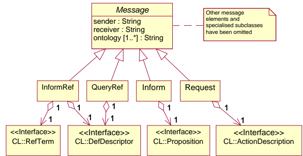
Figure 2: A partial UML model of an ACL
