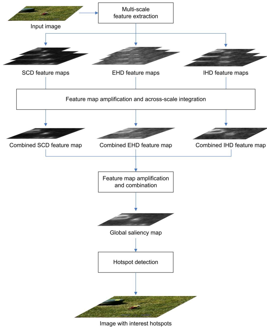
Figure 2: Diagram for hotspots detection.
