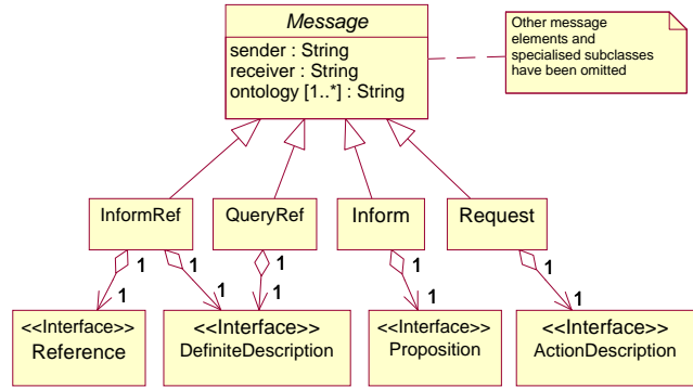
Figure 1: A UML class diagram for an agent communication language
