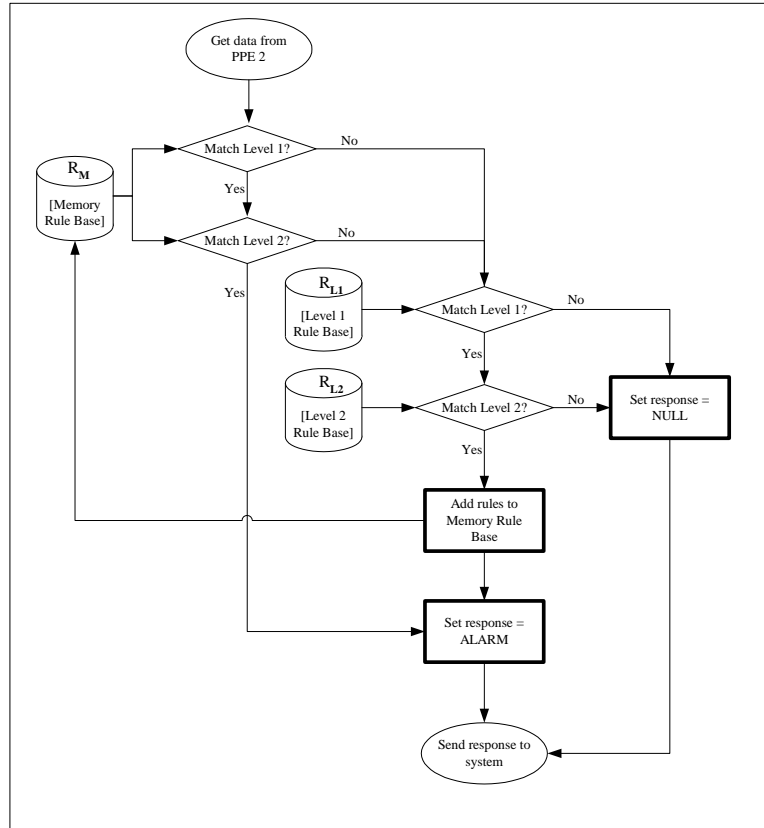
Fig. 2. Algorithm for the Adaptive Analysis Engine.
