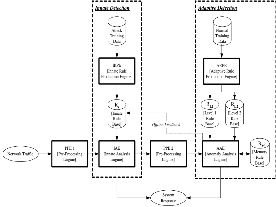
Fig. 1. Immune inspired intrusion detection framework.
